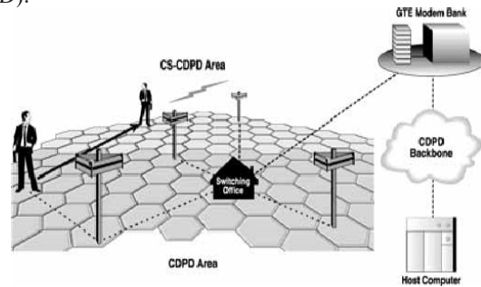
Fig.3 Circuit Switched CDPD
