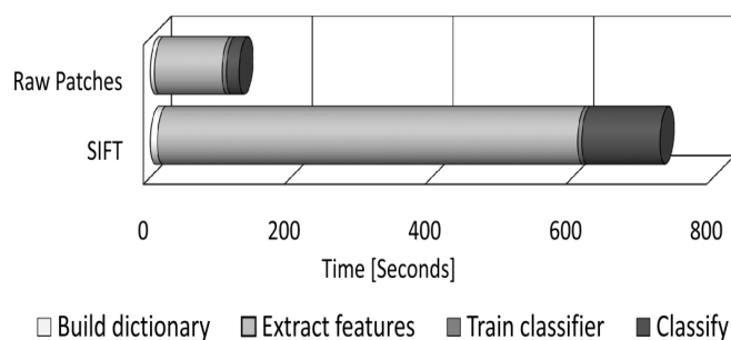
Fig.5 Running time using SIFT descriptors and normalized raw patches.
