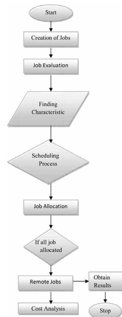
Fig. 2 Process flow of Job Allocation
