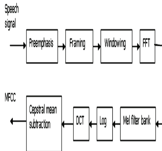
Fig.1Extraction of MFCC from speech signal
