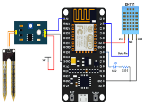
Fig. 7 Connection diagram
