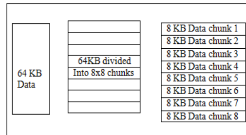
Fig. 1 Data Segmentation
