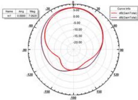
Fig. 4 Radiation pattern of proposed antenna at 4.7 GHz
