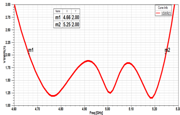
Fig. 3 Variation of VSWR v/s Frequency for proposed antenna
