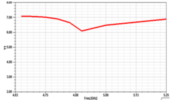
Fig. 7 Variation of directivity v/s frequency for Proposed antenna
