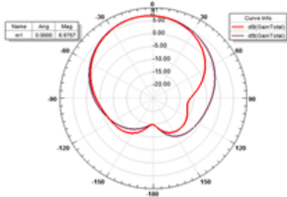
Fig.5 Radiation pattern of proposed antenna at 4.8 GHz
