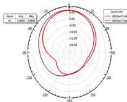
Fig. 6 Radiation pattern of proposed antenna at 5.2 GHz
