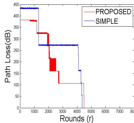
Fig. 17 Network path loss at EO = 0.5
