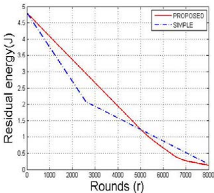
Fig. 14 Remaining energy at EO = 0.6
