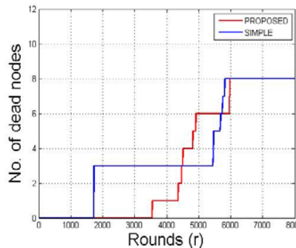
Fig. 4 Network lifetime at EO = 0.4
