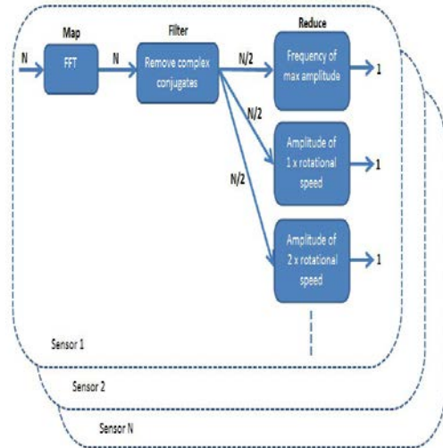
Fig. 3 Big Data Technique for reducing computation time
