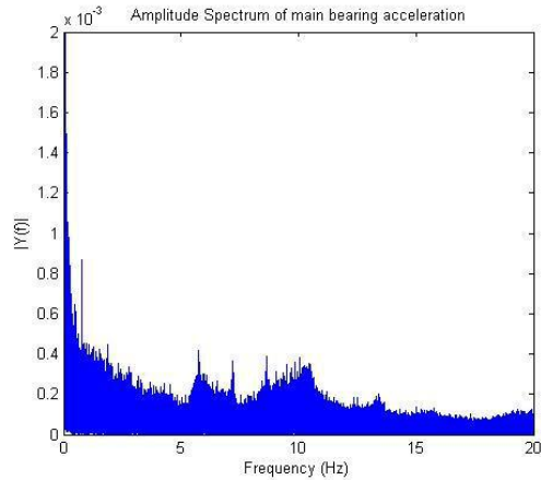
Fig. 1 Amplitude spectrum of main bearing acceleration
