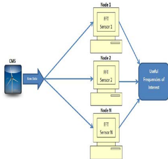
Fig. 4 Task sharing across multiple nodes
