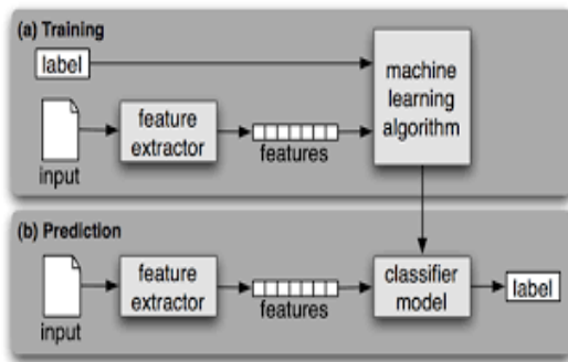
Fig. 1 Sentiment analysis basic architecture
