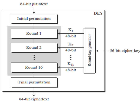
Fig. 3 General structure of DES
