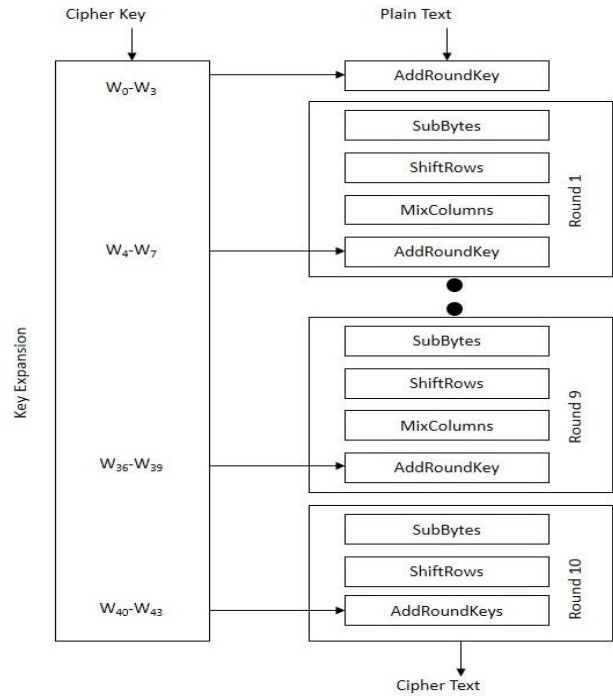
Fig. 4 AES Encryption flow [15].
