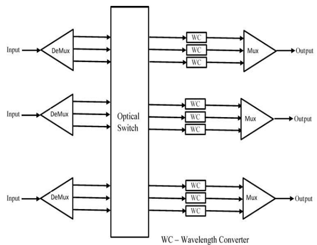
Fig. 1 Full wavelength converters architecture
