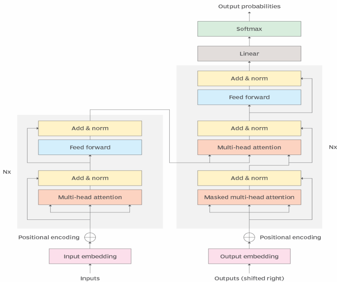
Fig. 2 A Transformer Model's Architecture Diagram
