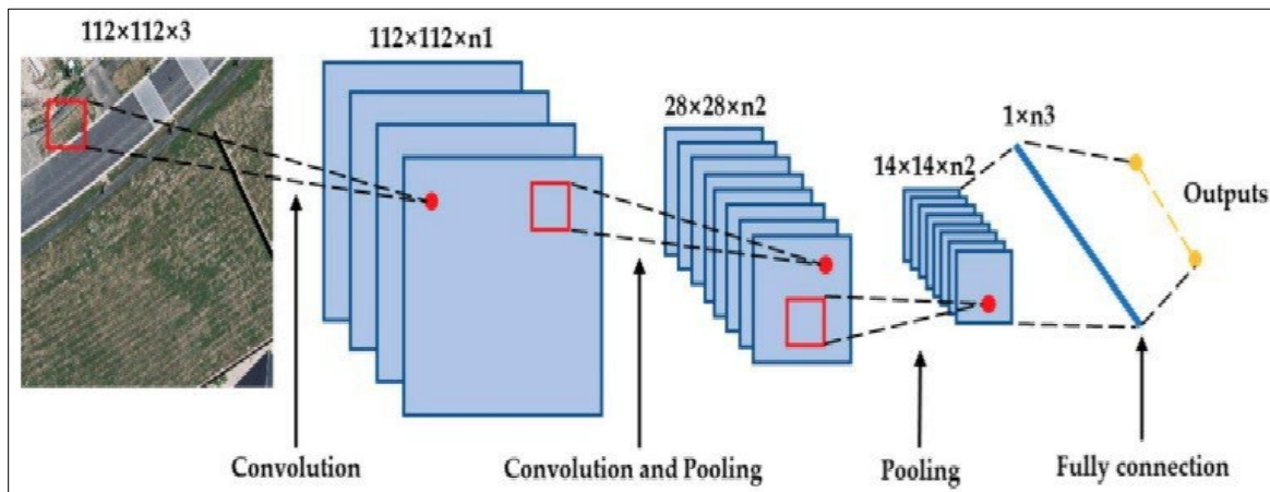
Fig. 1 CNN Architecture
