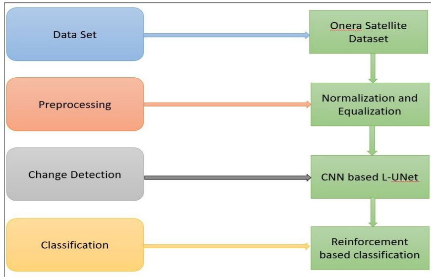
Fig. 3 Model Architecture
